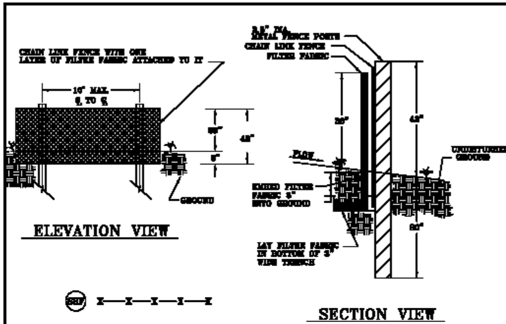
SUPER SILT FENCE NO SCALE
