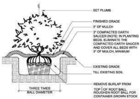
B SHRUB PLANTING NTS
