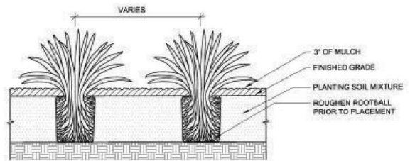
C PERENNIAL PLANTING NTS
