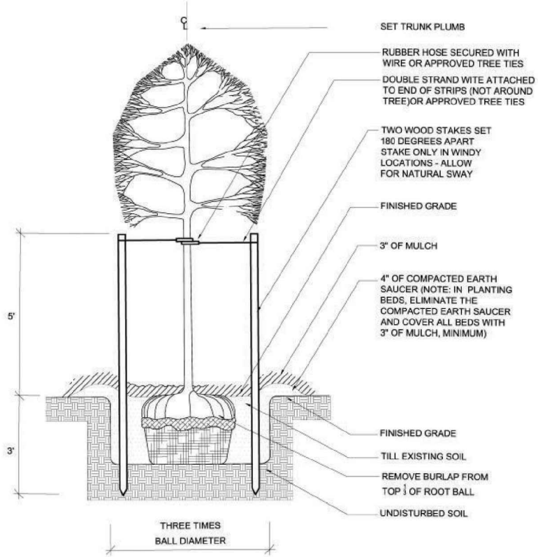
A TREE PLANTING NTS
