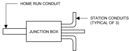
CORRECT INSTALLATION
