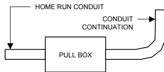
CORRECT INSTALLATION
