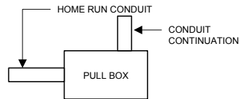
INCORRECT INSTALLATION
