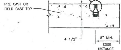
LIFTING INSERT DETAILS FOR TOPS @ GRADE
